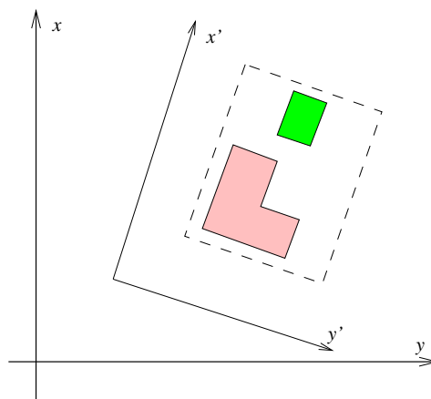
Figure 4: First example.
