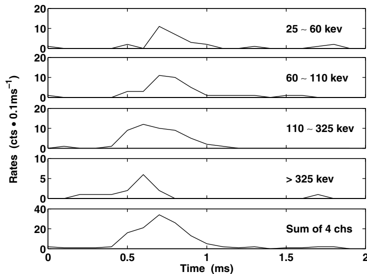
Figure 2. Counting rate profiles of a TGF with trigger number 2955 in different energy bands. From top to bottom is the profile in 25–60 keV, 60–110 keV, 110–325 keV, >325 keV and the total BATSE band, respectively.
