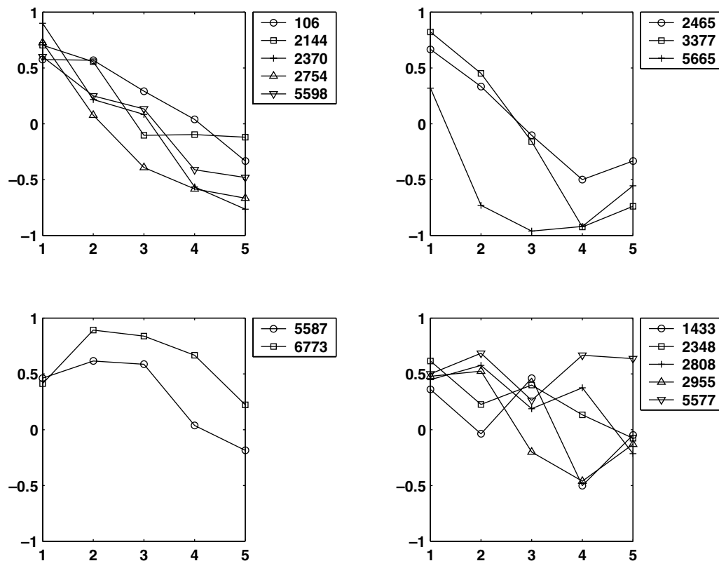
Figure 3. Spectral evolution of TGFs. The vertical axis is the hardness ratio defined by Eq. (3). The number marked along the abscissa is the segment number of a burst profile.
