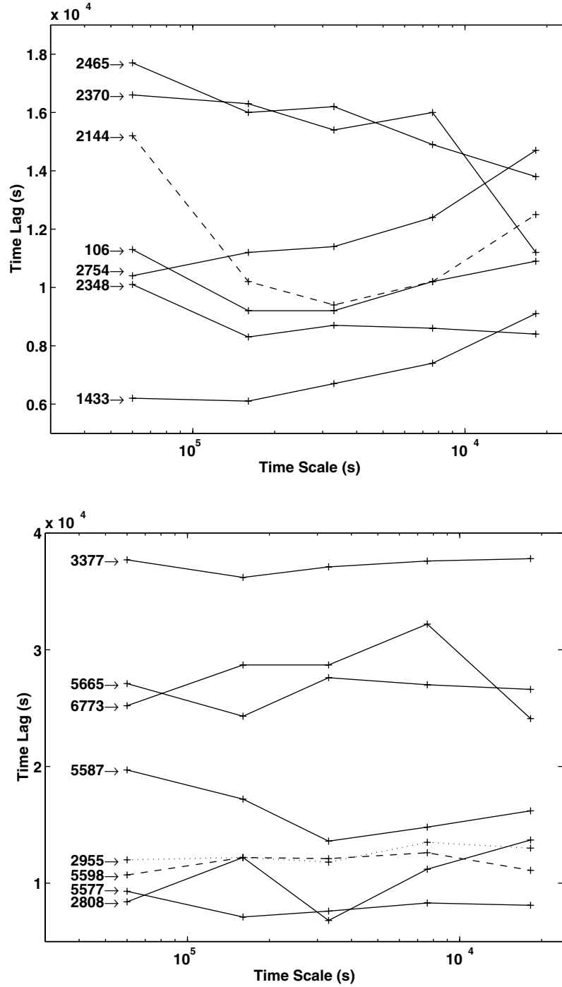
Figure 1. Soft \gamma -ray lag vs. time scale of TGFs. The quantity beside an arrow is the BATSE trigger number of the indicated burst.
