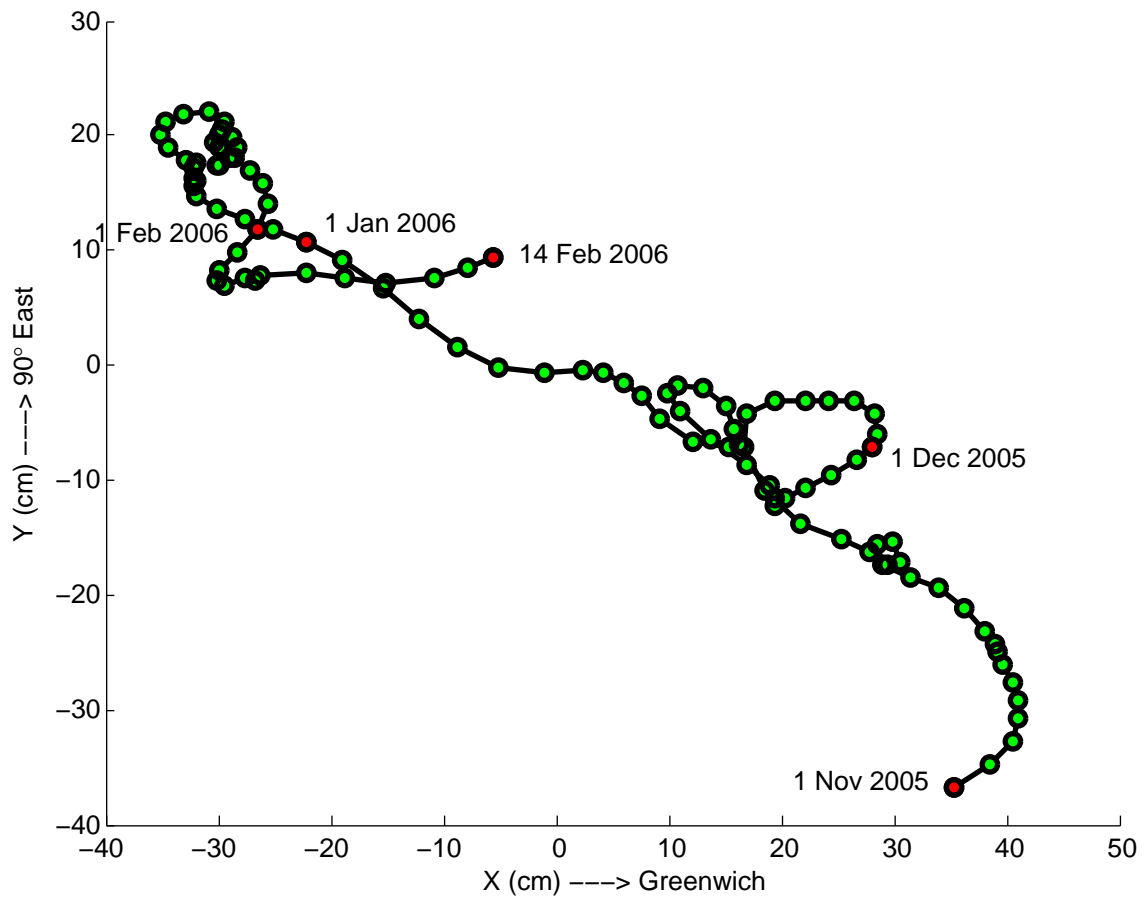
Motion of the North Pole, as determined by the IERS Earth Orientation Parameter Center of the Paris Observatory, for the study period, 1 November 2005 to 14 February 2006. Each marker represents the position of the pole on one day. Five loops are identified. Never before have these small polar movements been traced with such precision.
