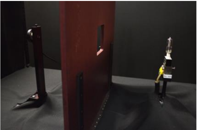
Figure 7. Transfer of standard from NIST lightbulb
